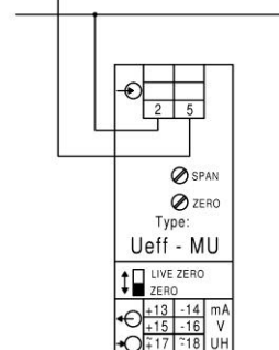
Spannungsmessung (TrueRMS) voltage measuring (TrueRMS)
