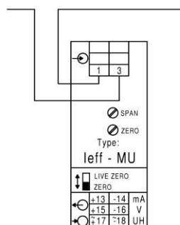
Strommessung (TrueRMS) current measuring (TrueRMS)
